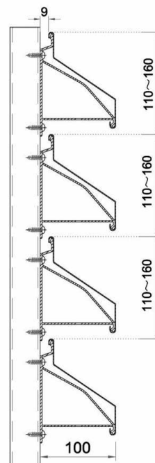
CZ132-SIDE VIEW
