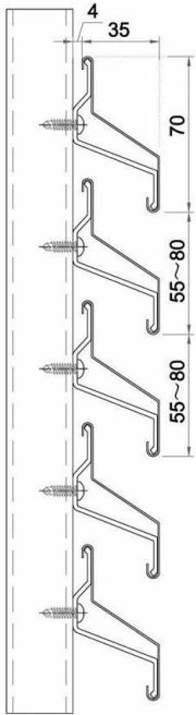
CZ70-SIDE VIEW
