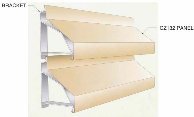
ISOMETRIC DETAILS
