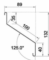
CZ132-PRODUCT DETAILS
